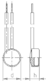
Diameter d 9,4 mm Installation height h from 5,4 mm
